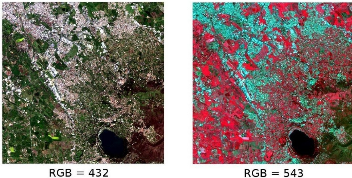
Abb. 4: Color composite of a Landsat 8 image Data available from the U.S. Geological Survey
