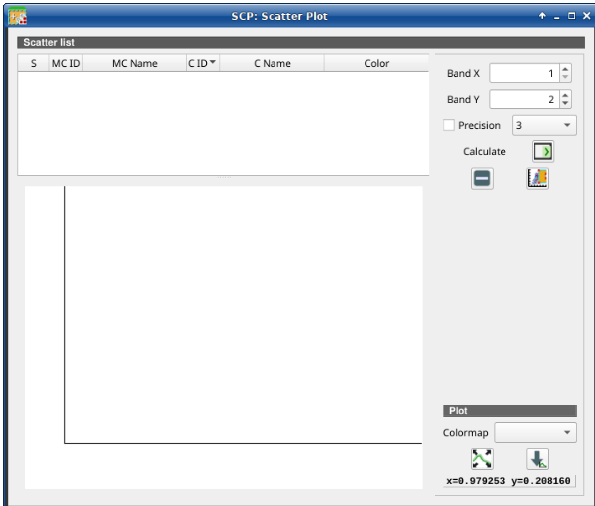
Abb. 54: Scatter Plot
