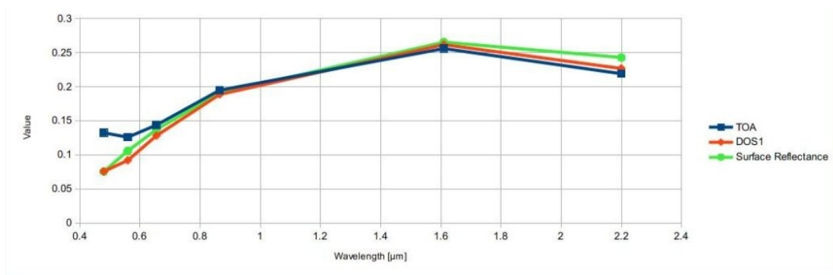
Abb. 13: Spectral signatures of a built-up pixel
