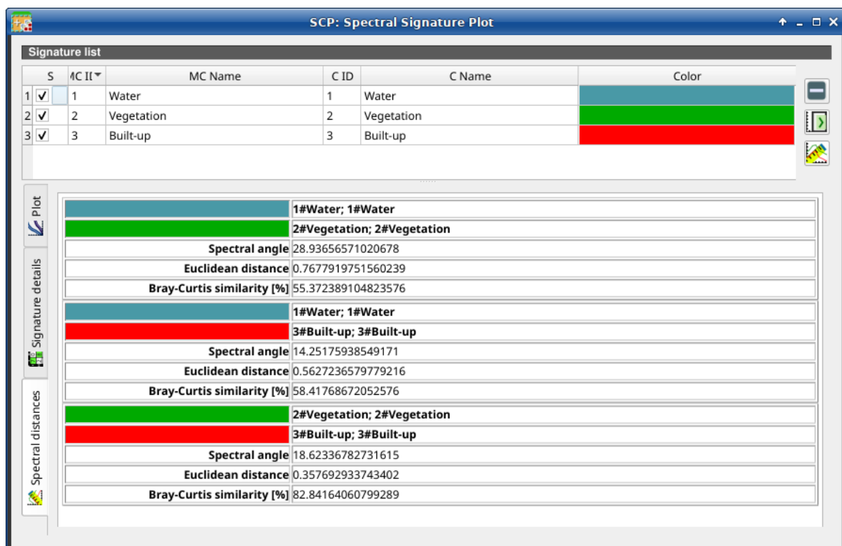
Abb. 53: Spectral Signature: Example of spectral distances
