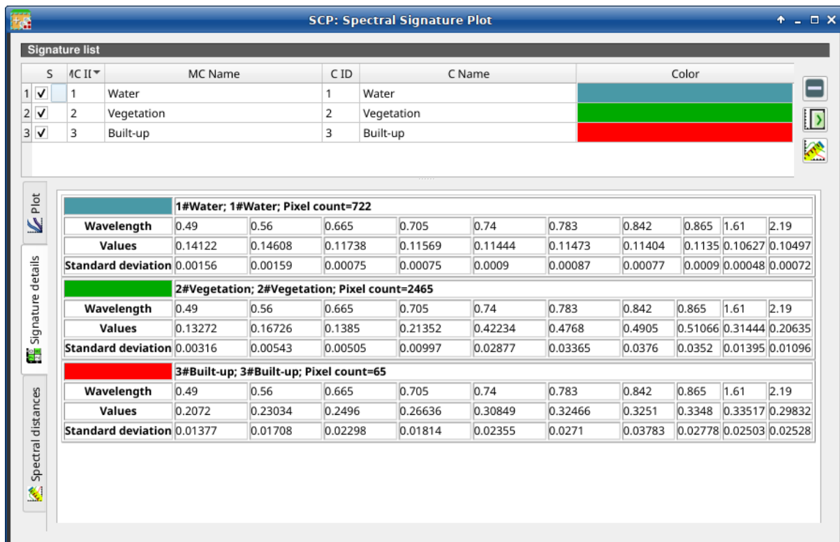
Abb. 52: Spectral Signature: Example of signature details
