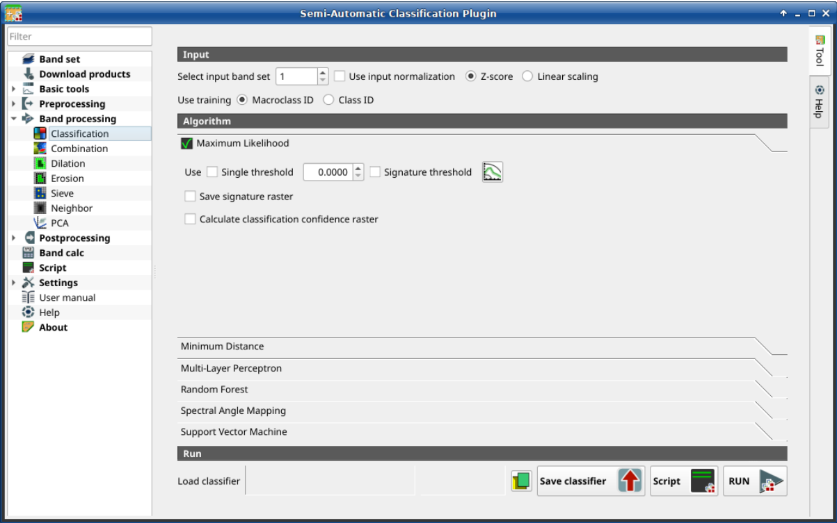
Abb. 28: Maximum Likelihood
