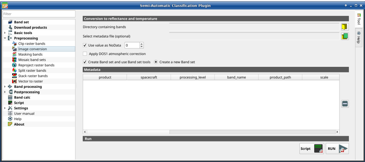
Abb. 20: Image conversion
