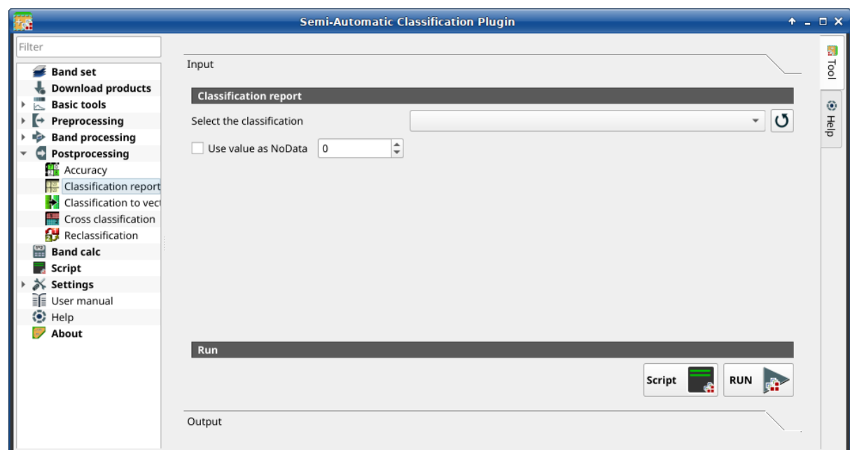
Abb. 41: Classification report
