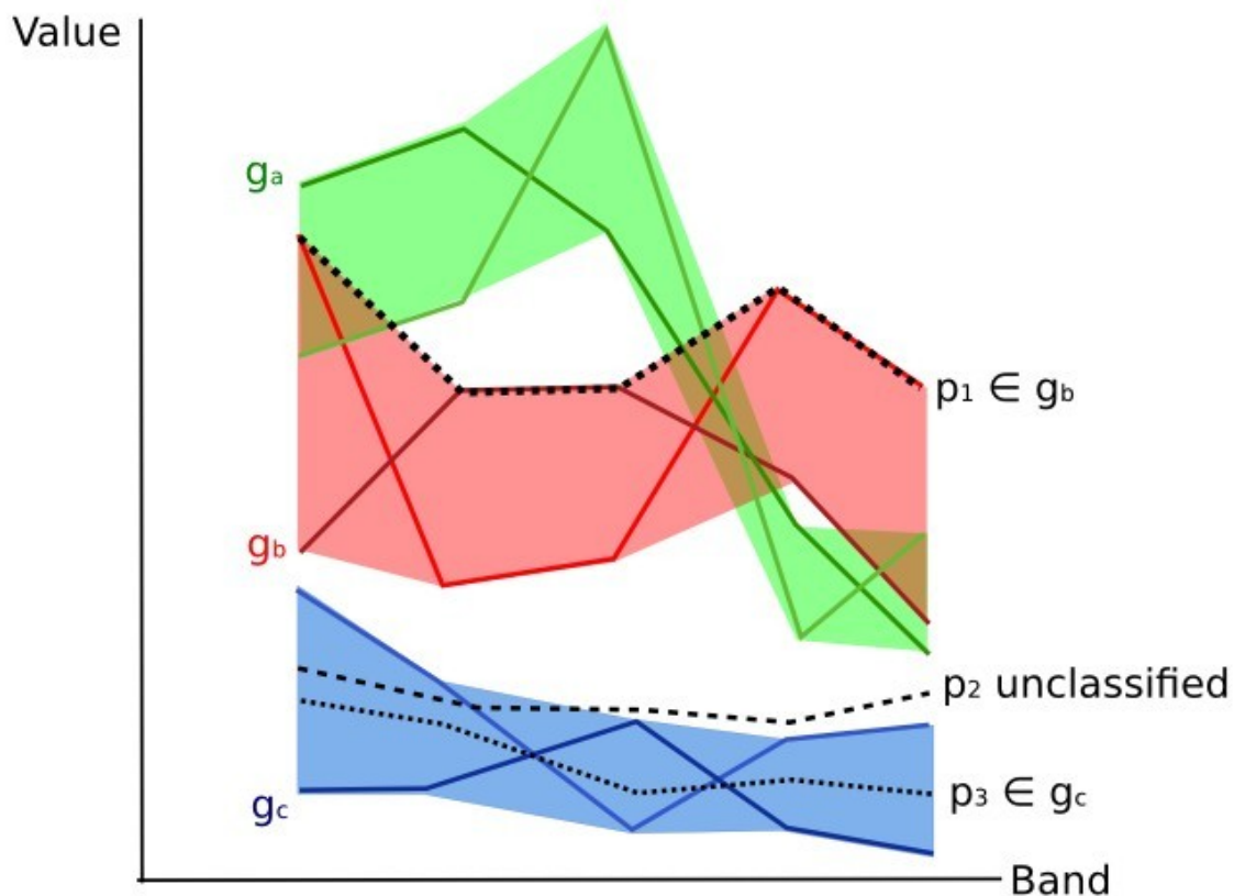
Abb. 10: Plot of spectral ranges
