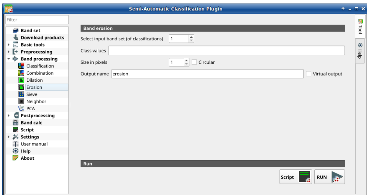
Abb. 36: Erosion
