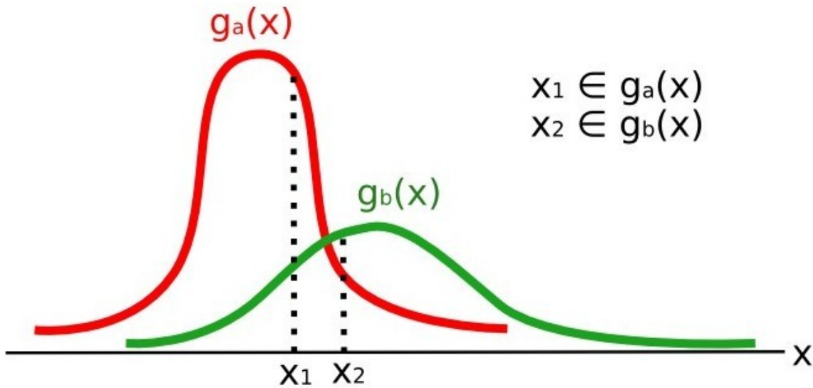
Abb. 7: Maximum Likelihood example
