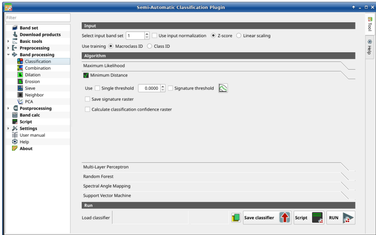
Abb. 29: Minimum Distance
