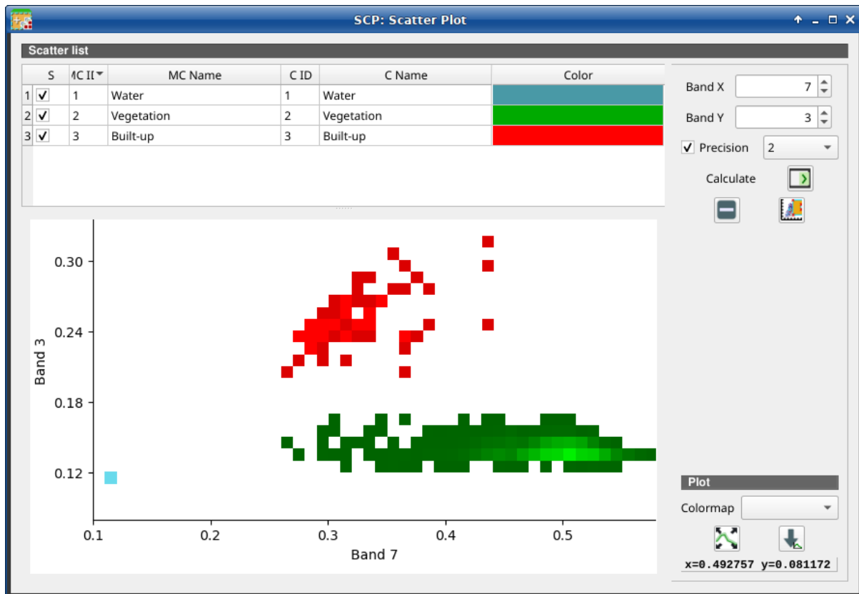
Abb. 55: Example Scatter Plot
