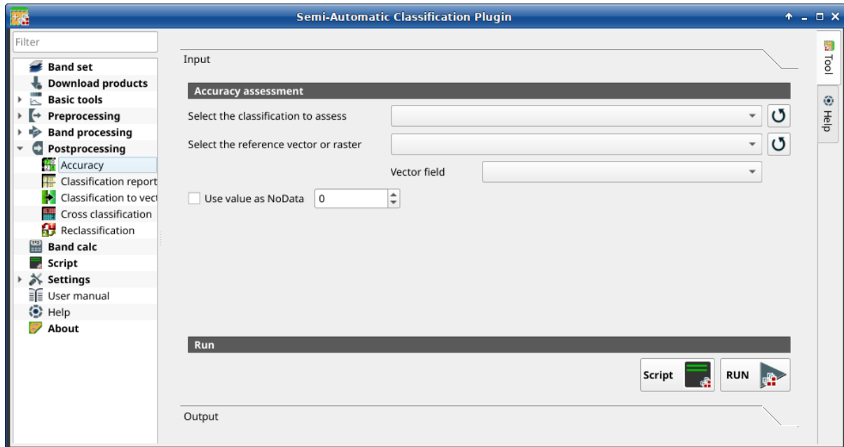
Abb. 40: Accuracy
