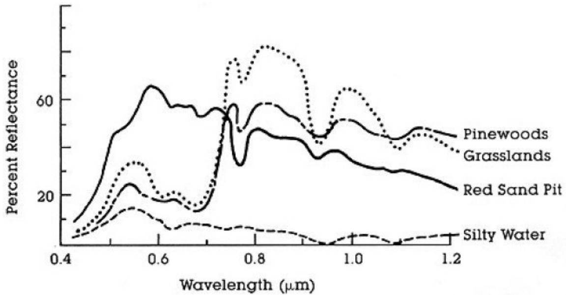
Abb. 2: Spectral Reflectance Curves of Four Different Targets (from NASA, 2013)
