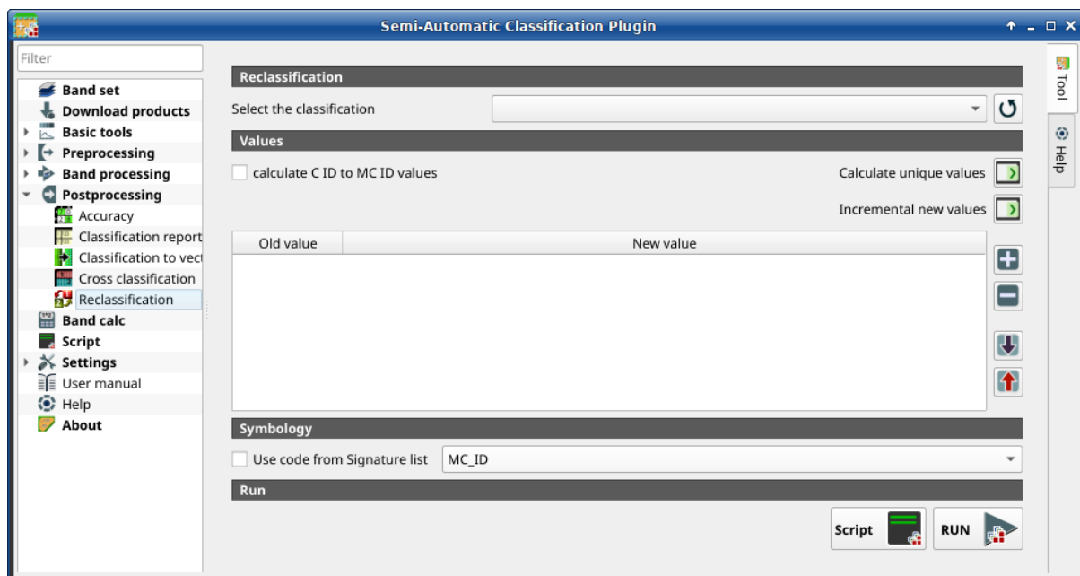
Abb. 44: Reclassification
