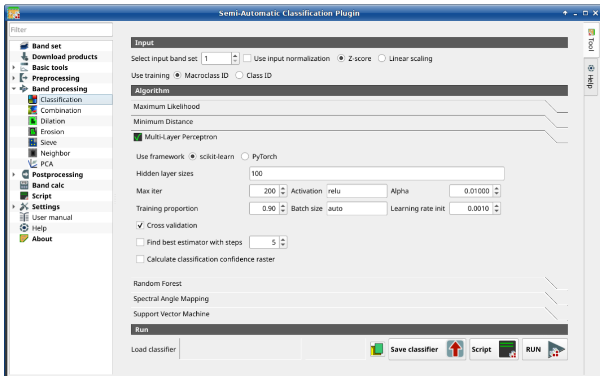
Abb. 30: Multi-layer Perceptron
