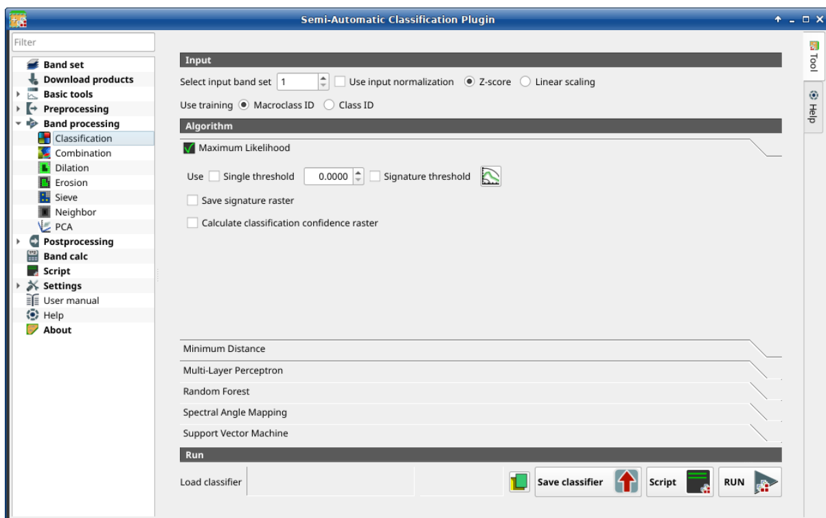
Abb. 27: Classification
