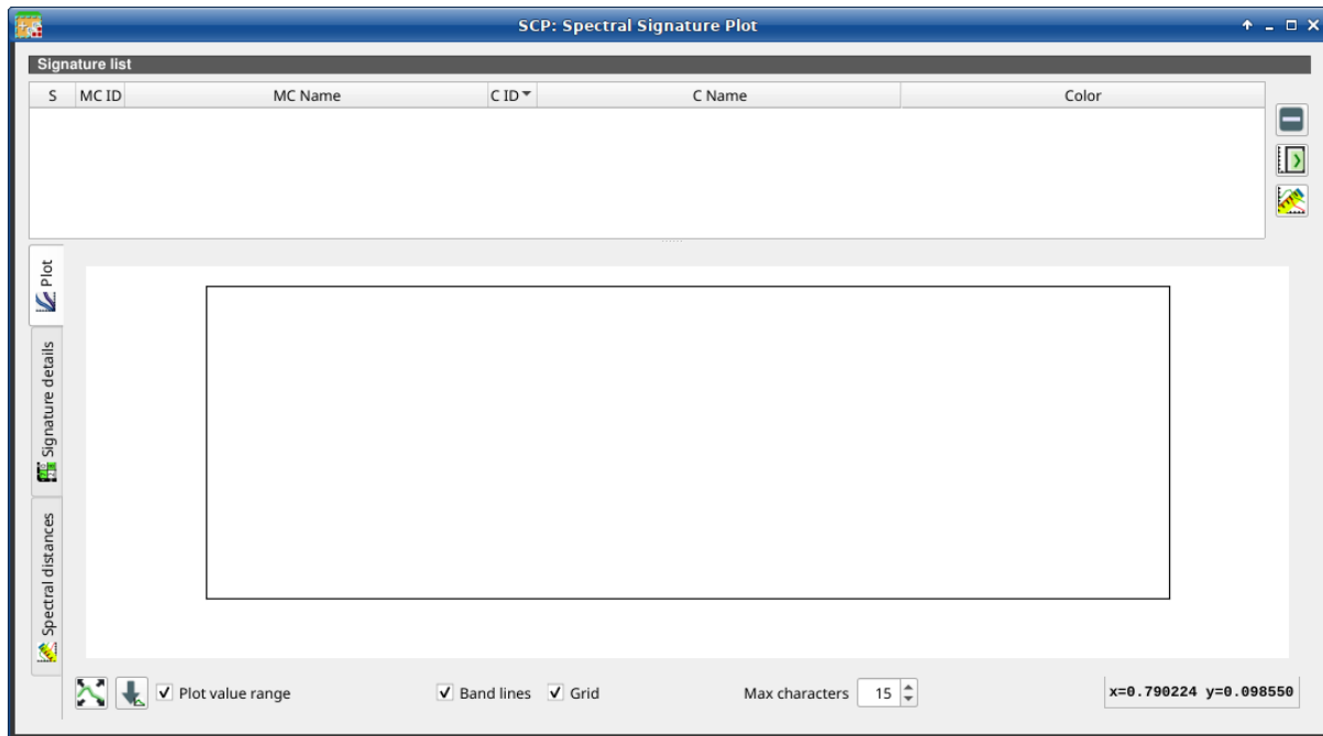
Abb. 50: Spectral Signature Plot
