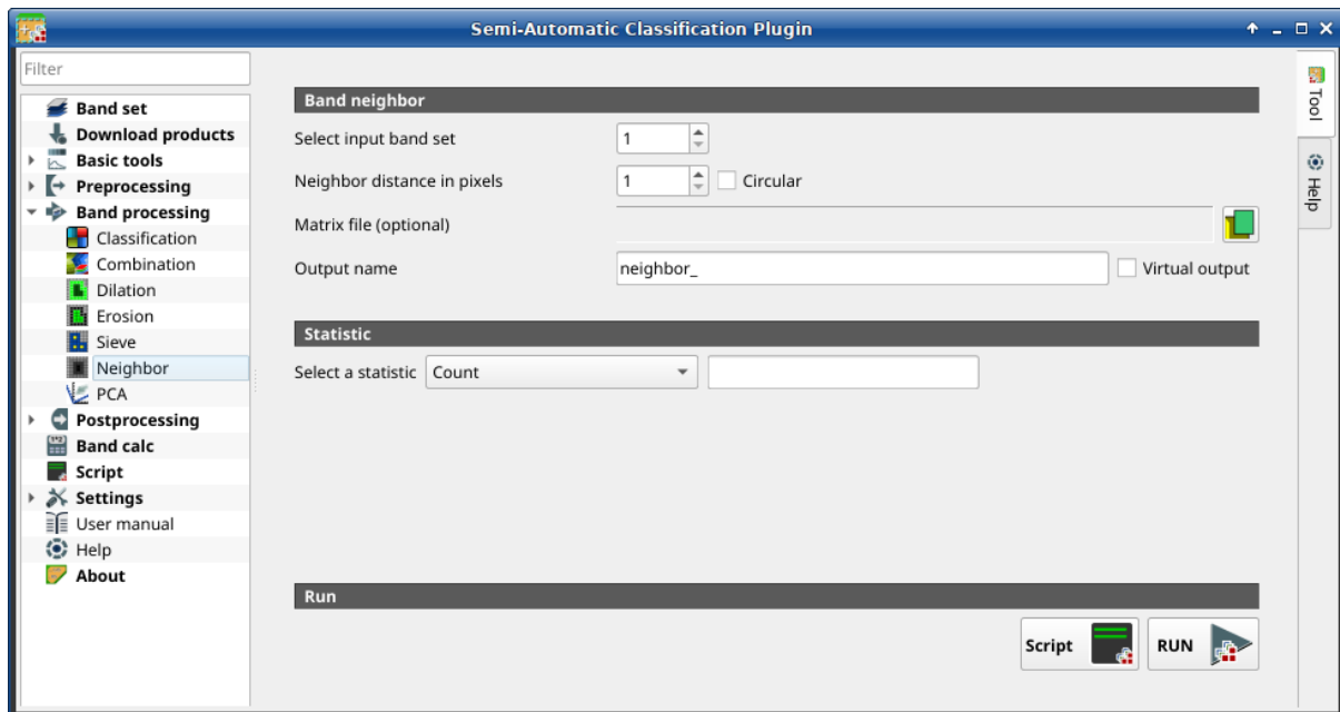
Abb. 38: Neighbor
