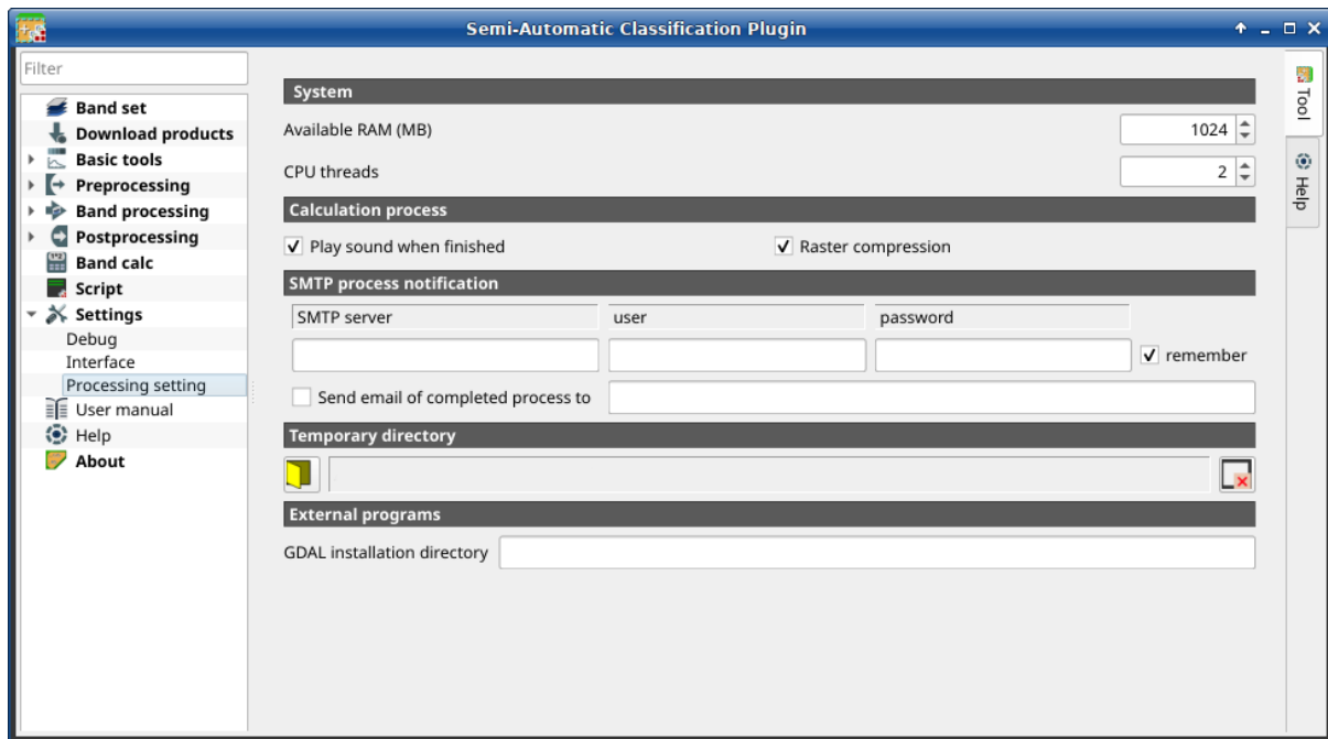
Abb. 49: Processing
