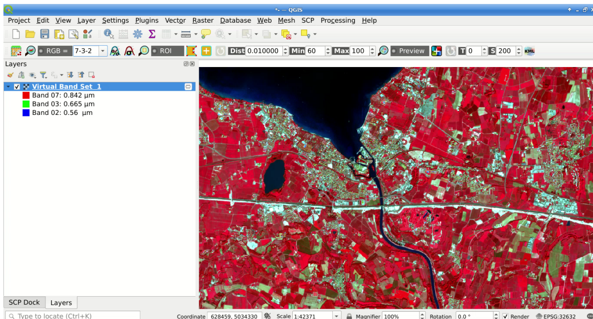
Abb. 2: Color composite RGB=7-3-2
