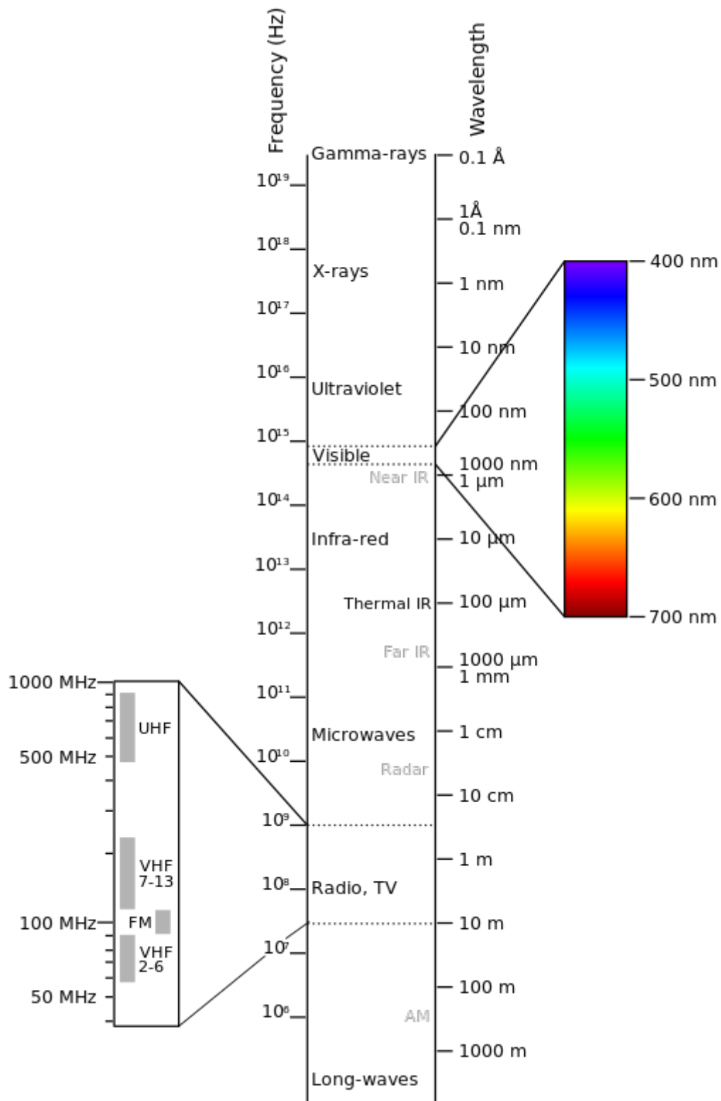
Abb. 1: Electromagnetic-Spectrum
