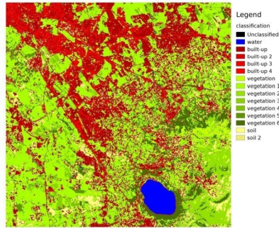
Abb. 11: Landsat classification Data available from the U.S. Geological Survey
