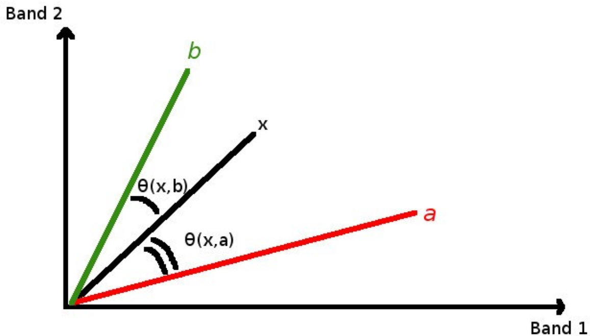
Abb. 8: Spectral Angle Mapping example
