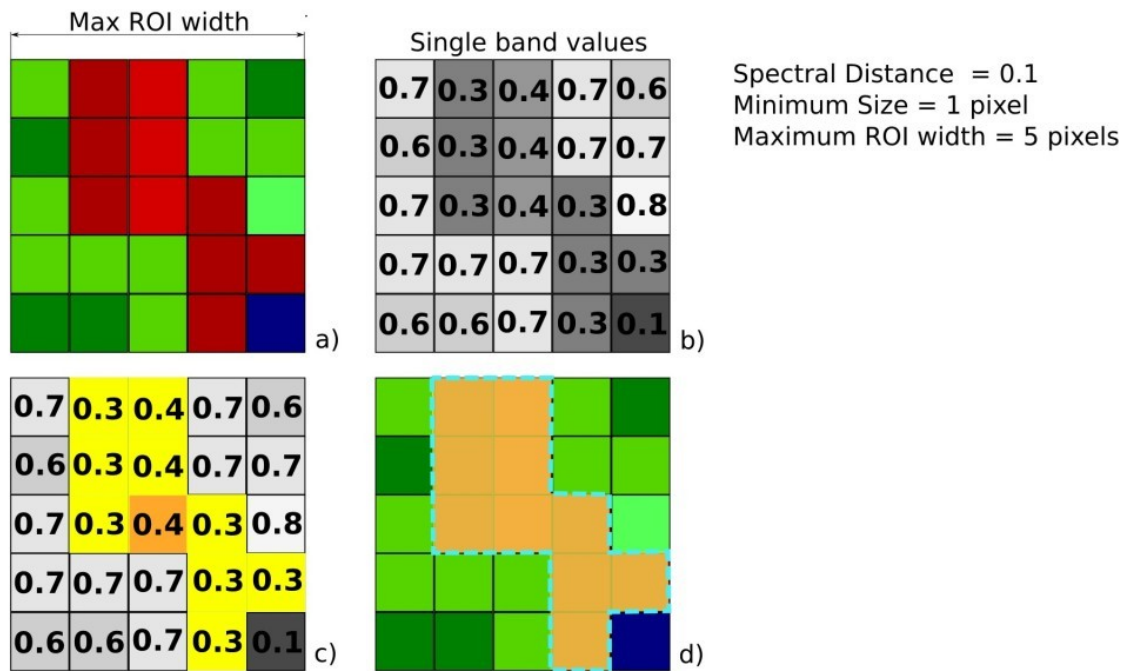
Abb. 5: Region growing example
