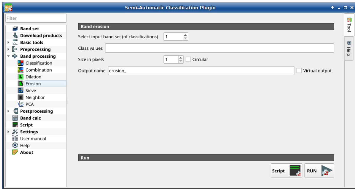
Gambar. 36: Erosi
