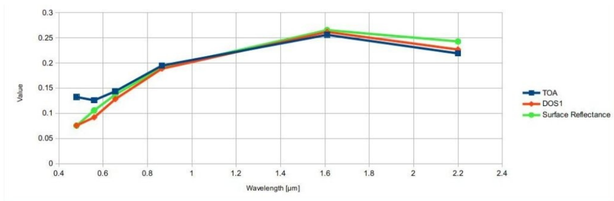
Gambar. 13: Spectral signatures of a built-up pixel
