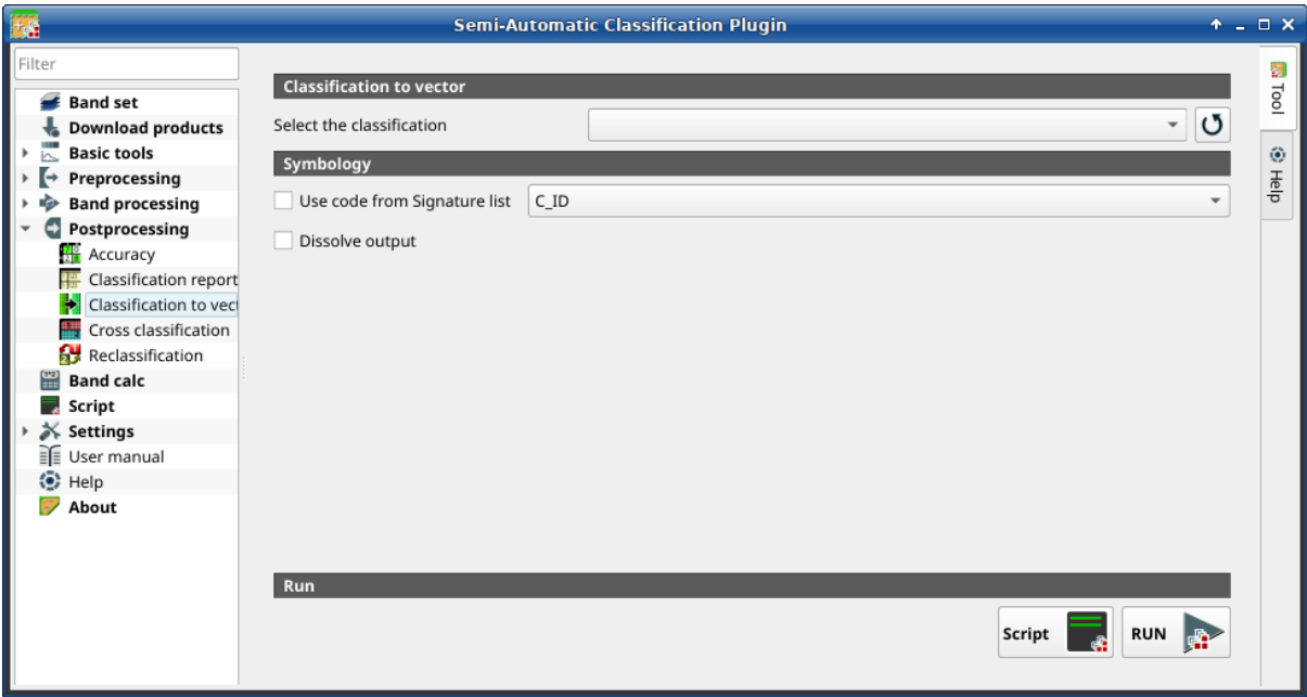
Gambar. 42: Classification to vector
