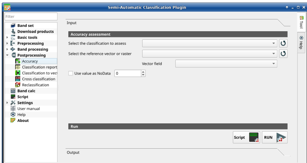
Gambar. 40: Accuracy
