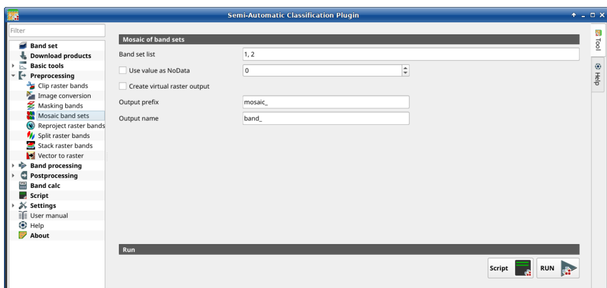
Gambar. 22: Mosaic band sets
