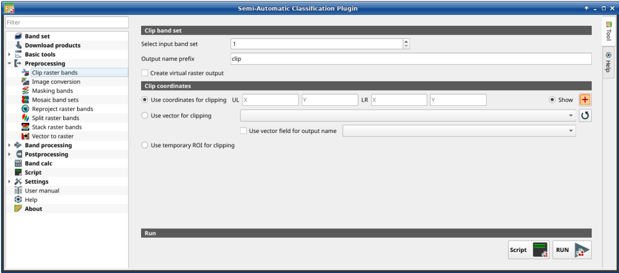
Gambar. 19: Clip multiple rasters
