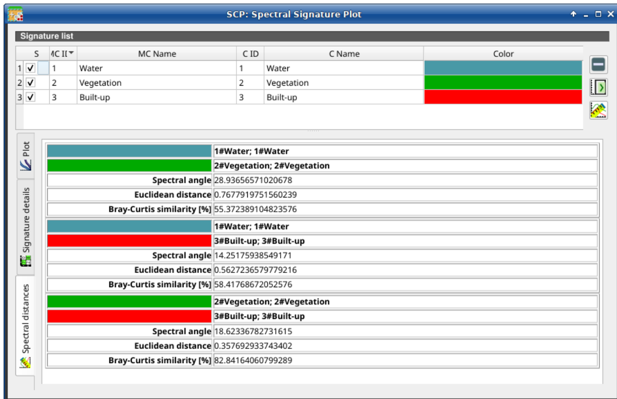
Gambar. 53: Spectral Signature: Example of spectral distances
