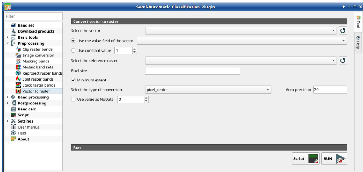
Gambar. 26: Vector to raster
