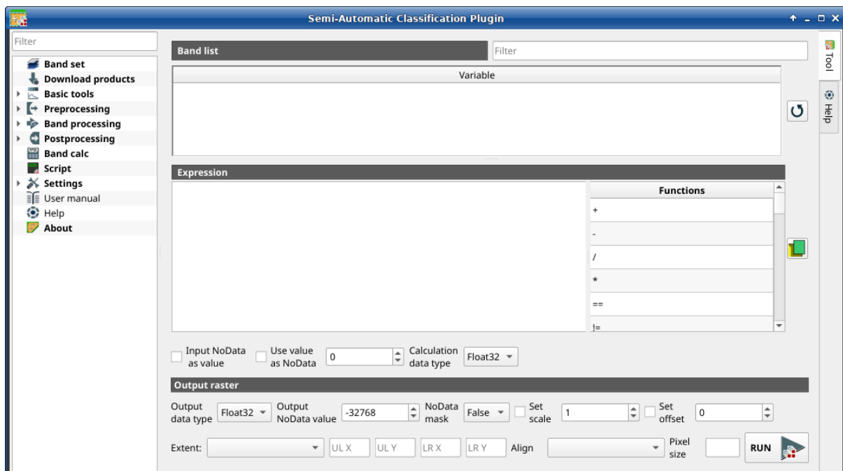
Gambar. 45: Band calc
