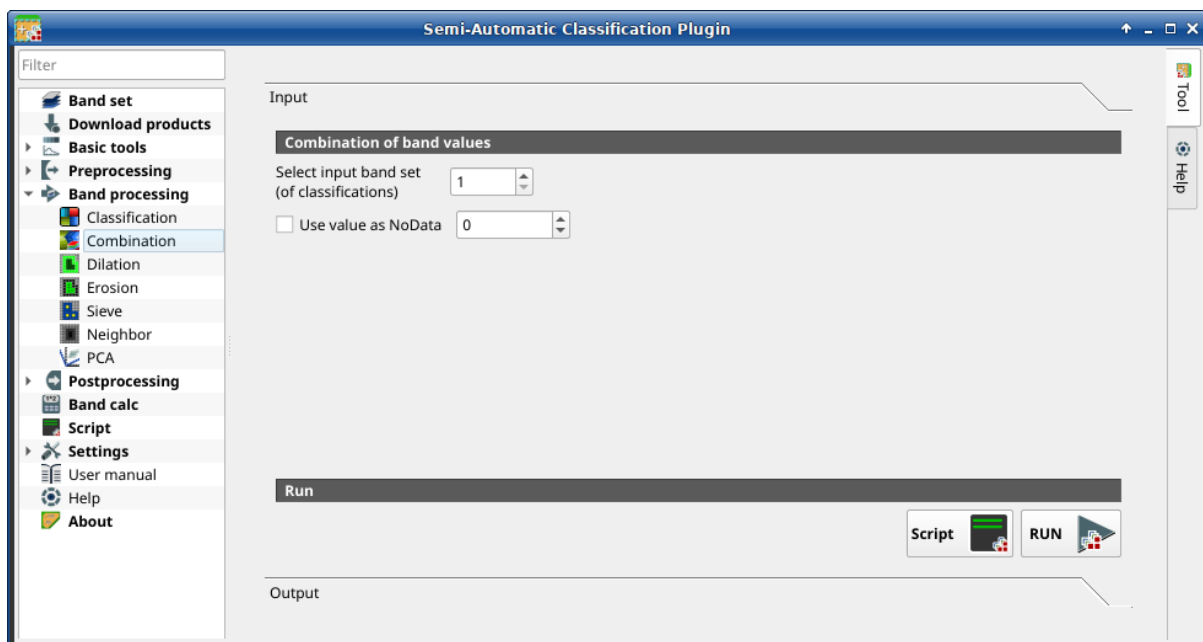
Gambar. 34: Combination
