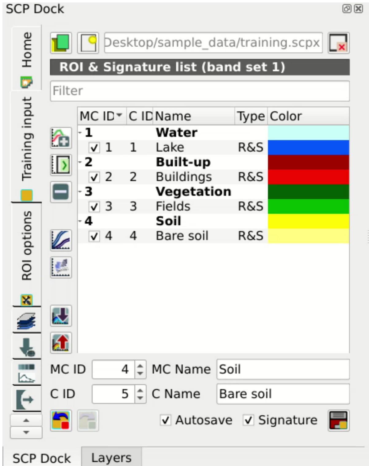
Gambar. 10: Definition of class colors
