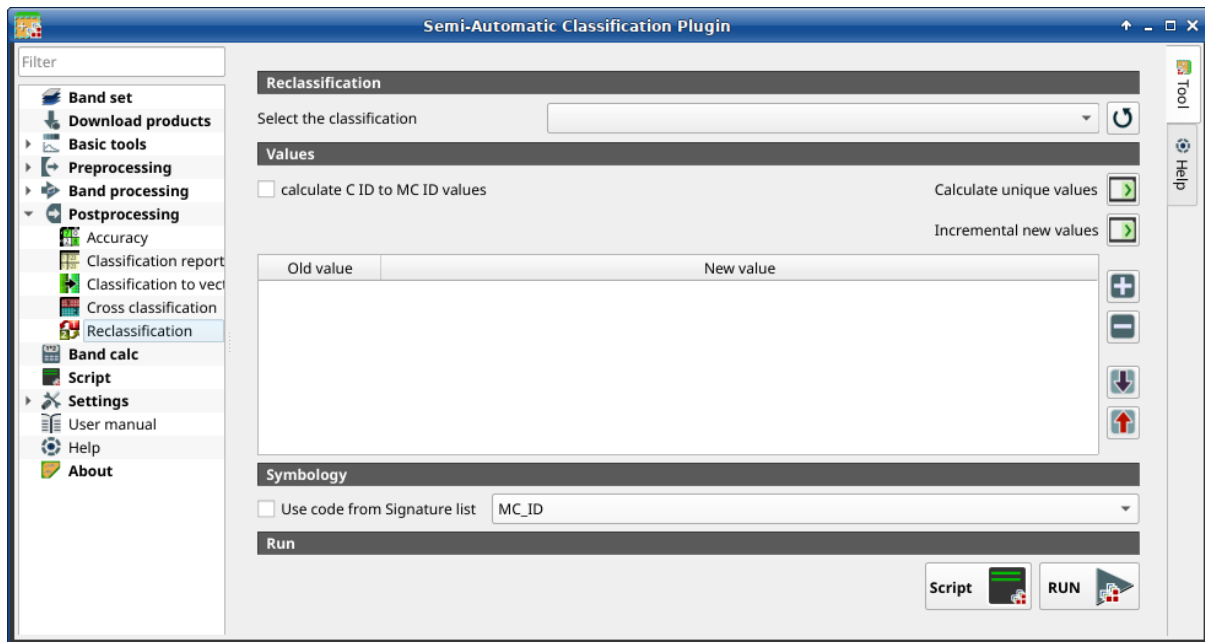
Gambar. 44: Reclassification
