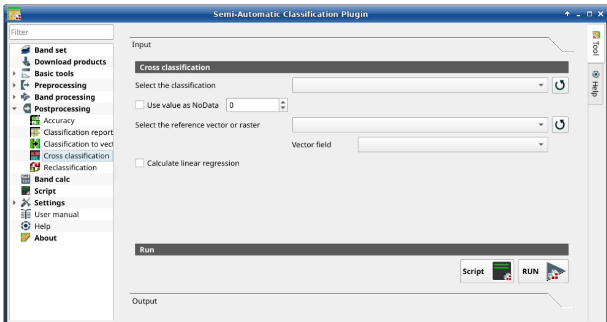
Gambar. 43: Cross classification
