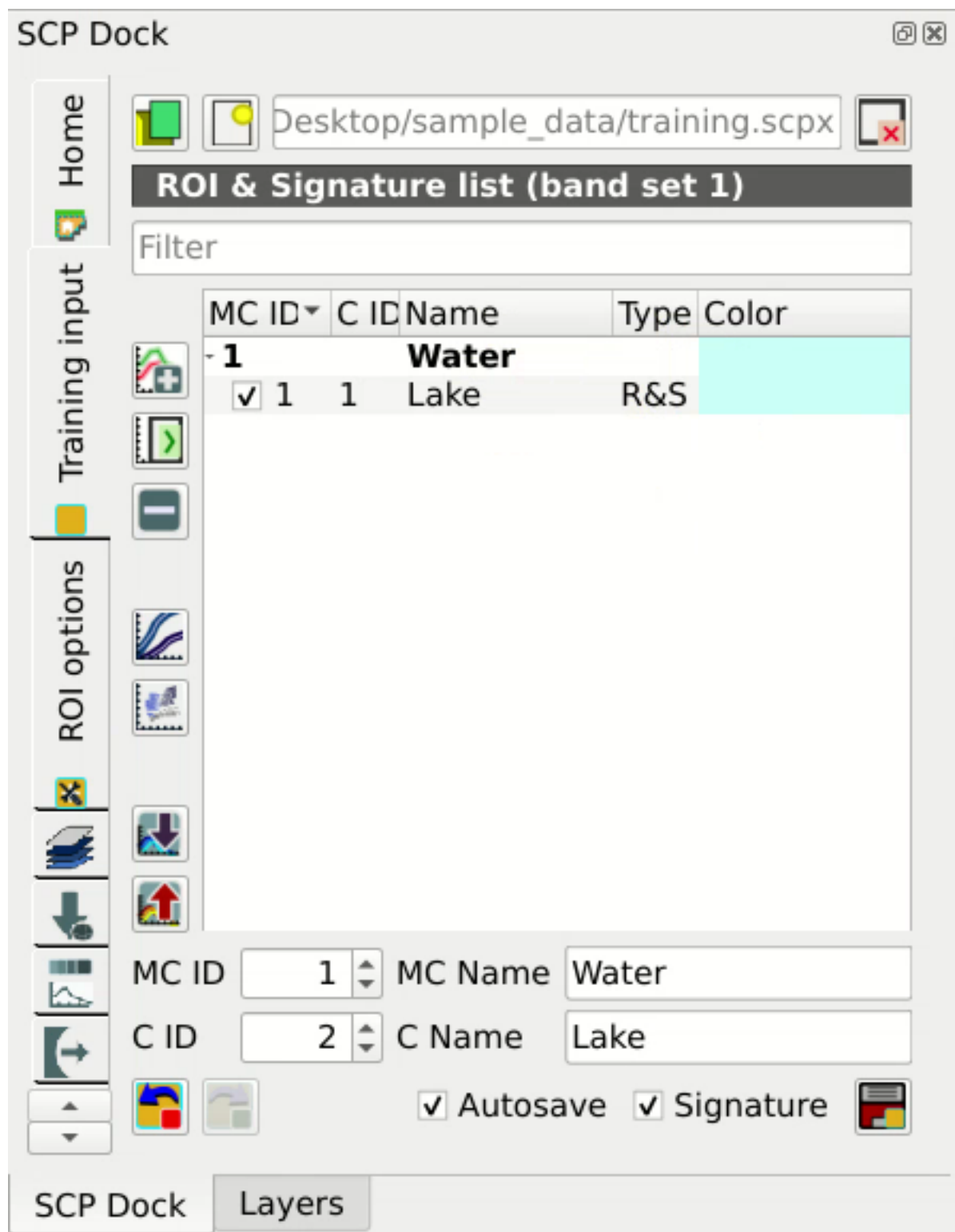
Gambar. 5: The ROI saved in the Training input
