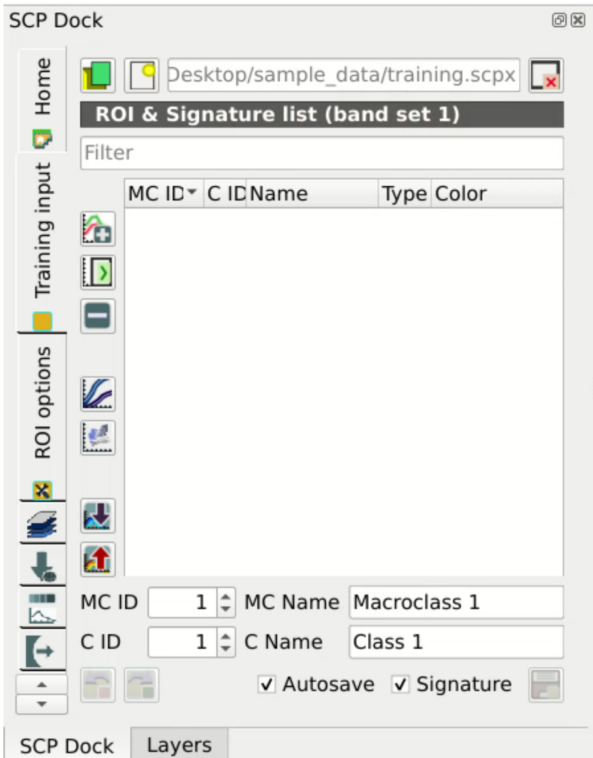
Gambar. 3: Definition of Training input in SCP
