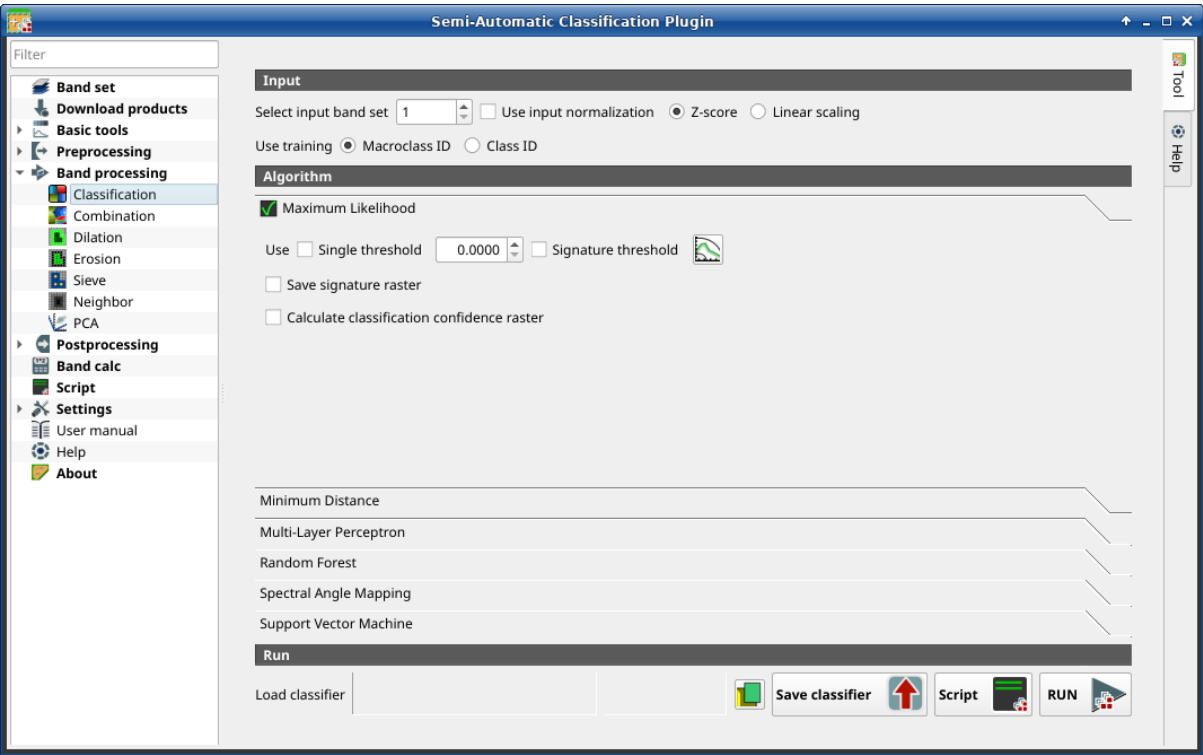
Gambar. 28: Maximum Likelihood
