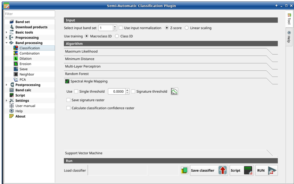
Gambar. 32: Spectral Angle Mapping
