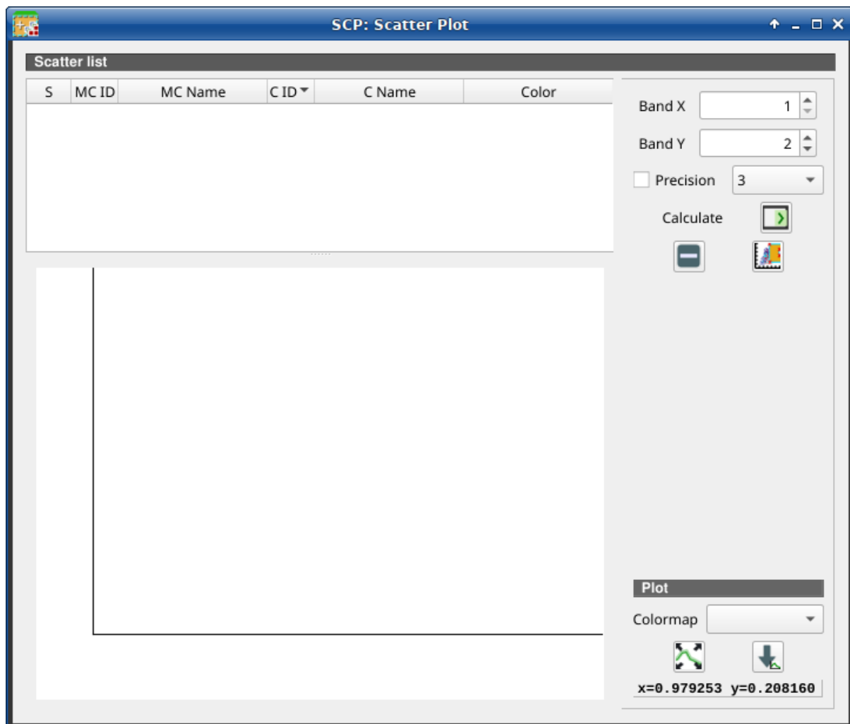
Gambar. 54: Scatter Plot
