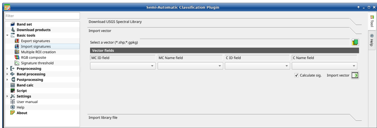
Gambar. 14: Import vector
