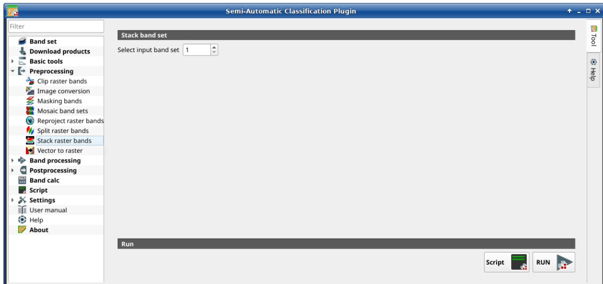
Gambar. 25: Stack raster bands
