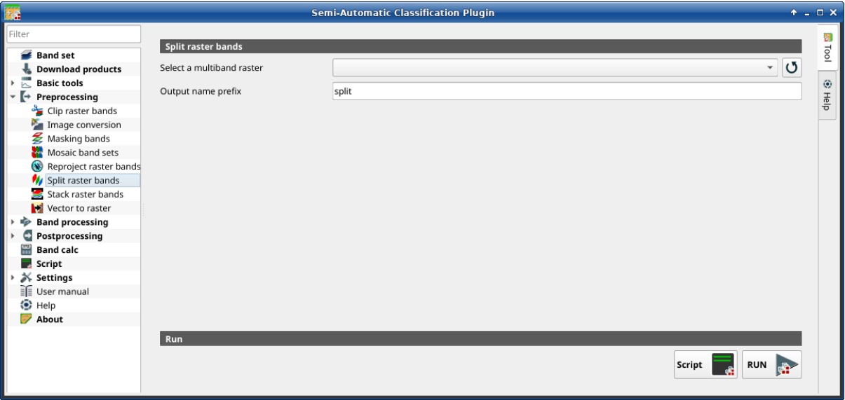
Gambar. 24: Split raster bands
