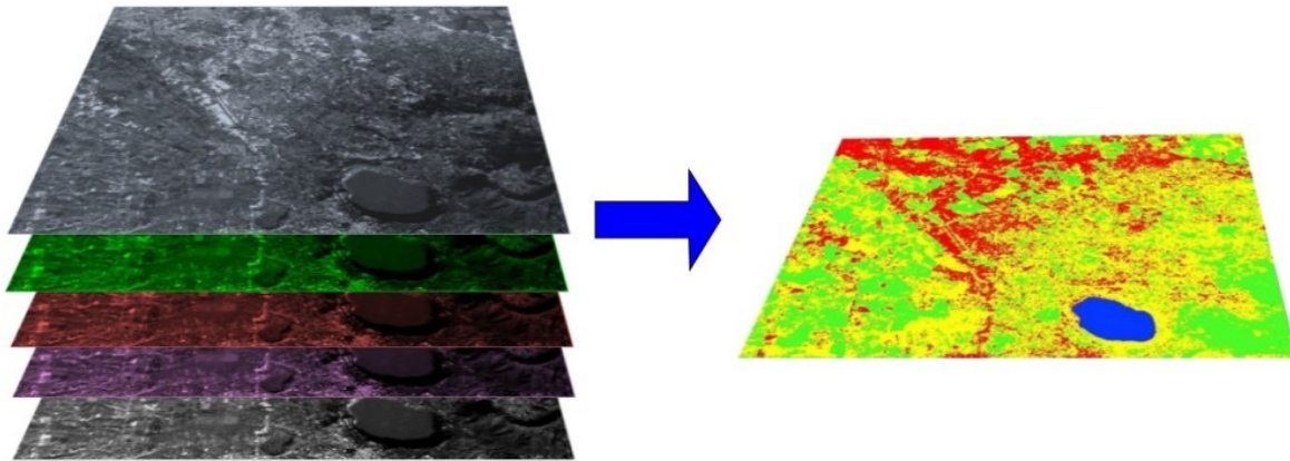
Gambar. 3: A multispectral image processed to produce a land cover classification "(Citra Landsat disediakan oleh USGS)"
