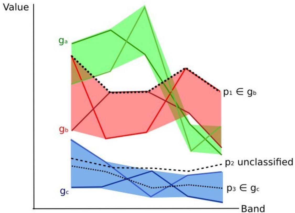
Gambar. 10: Plot of spectral ranges
