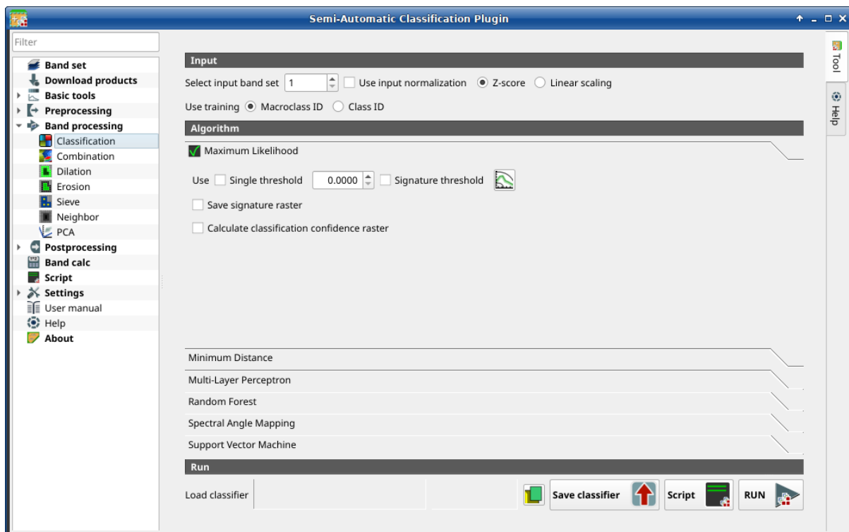
Gambar. 27: Classification
