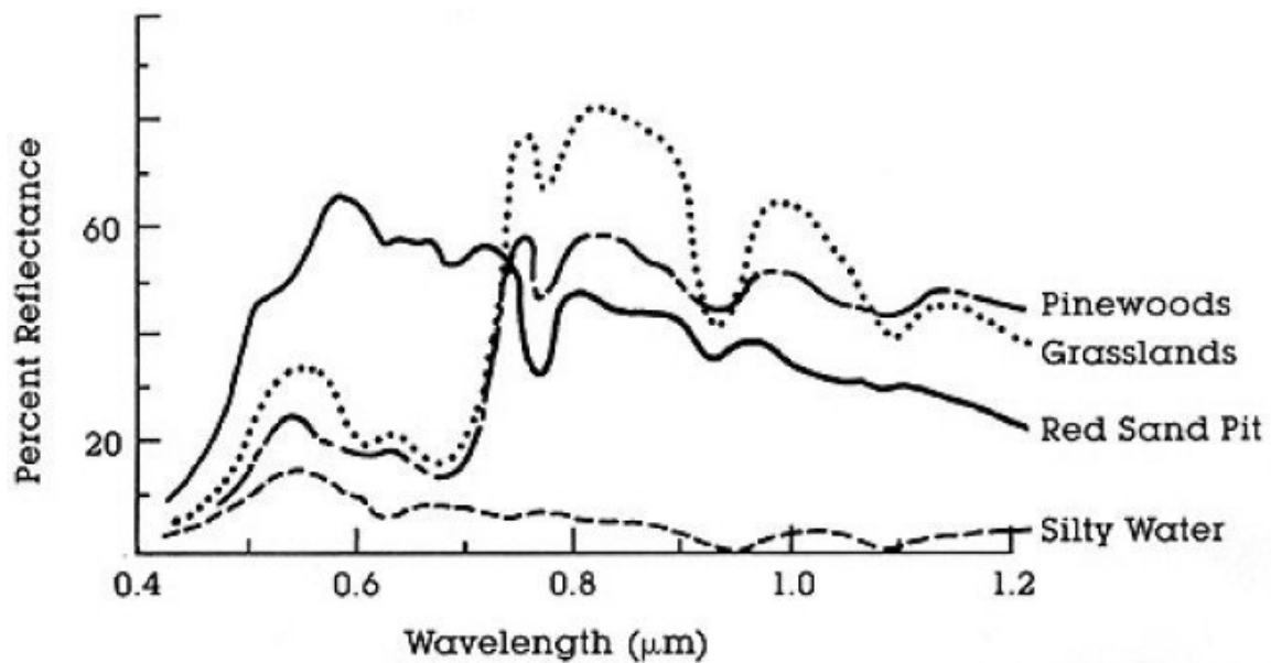
Gambar. 2: Spectral Reflectance Curves of Four Different Targets (from NASA, 2013)
