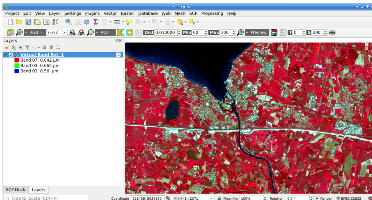
Gambar. 2: Color composite RGB=7-3-2
