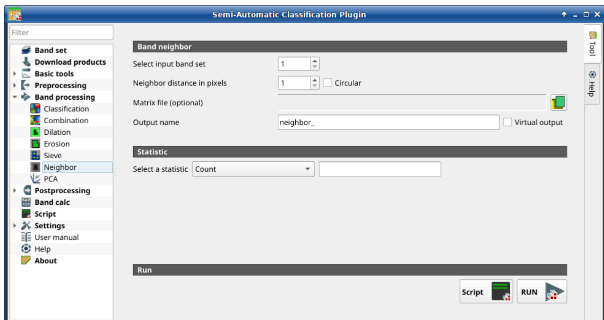
Gambar. 38: Neighbor
