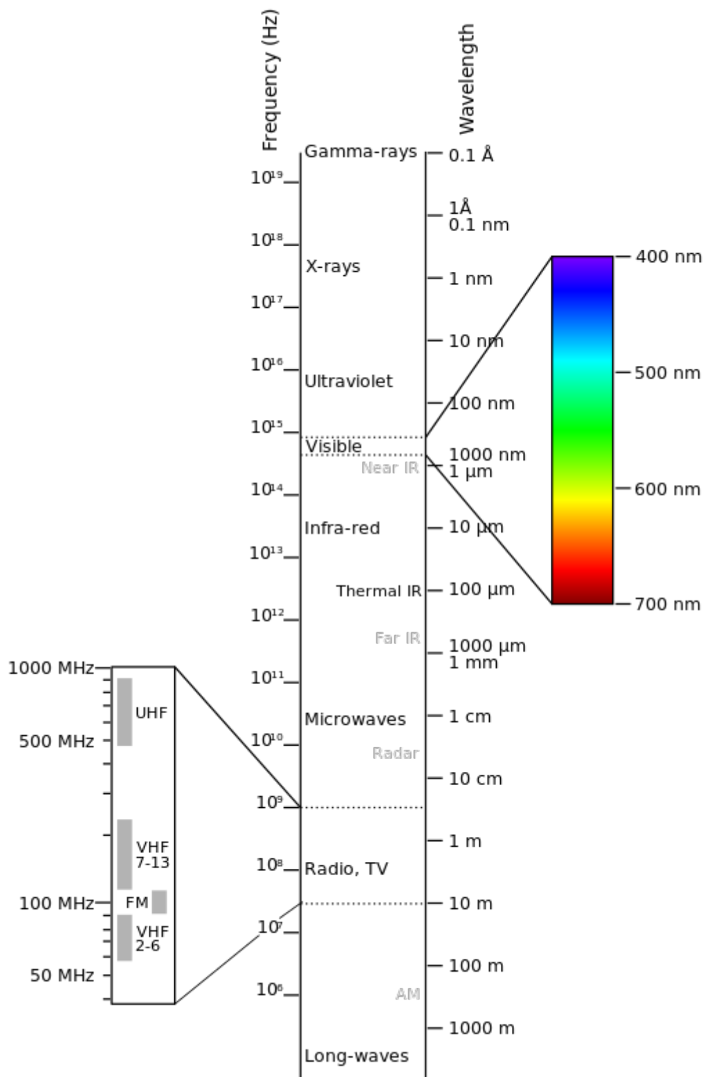
Gambar. 1: Electromagnetic-Spectrum
