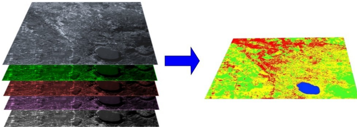
Gambar. 3: A multispectral image processed to produce a land cover classification (Landsat image provided by USGS)
