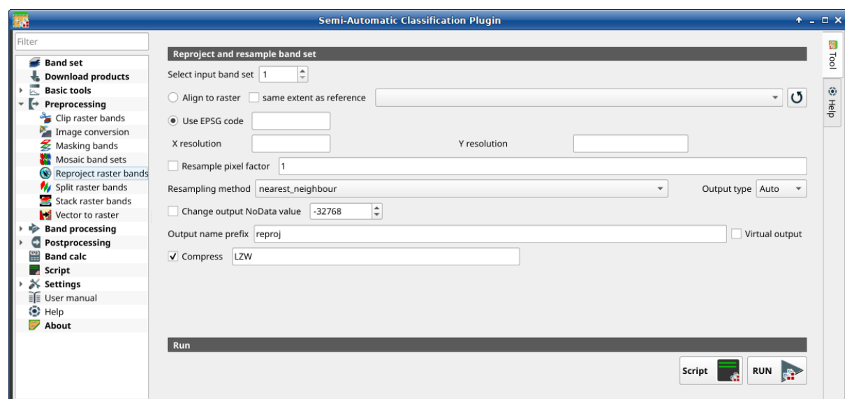
Gambar. 23: Reproject raster bands
