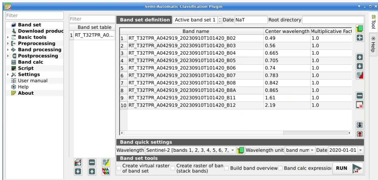
Gambar. 1: Definition of a band set
