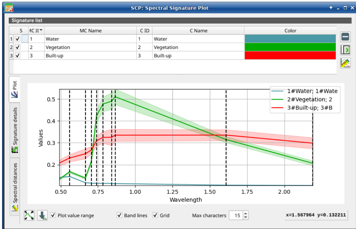
Gambar. 51: Spectral Signature: Example of plot
