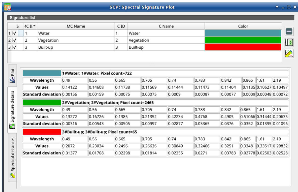
Gambar. 52: Spectral Signature: Example of signature details
