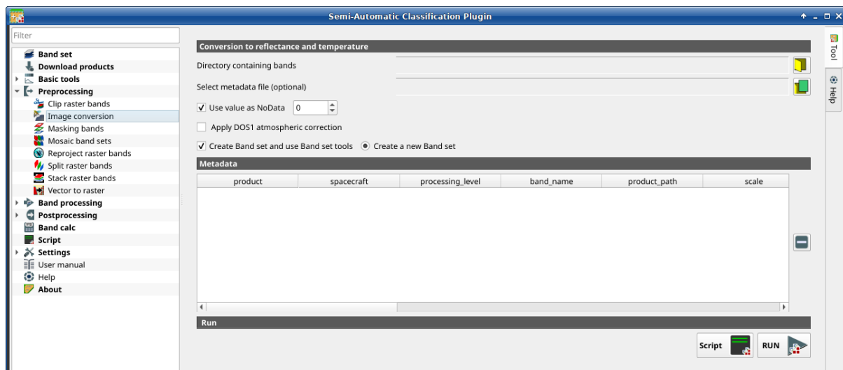
Gambar. 20: Image conversion
