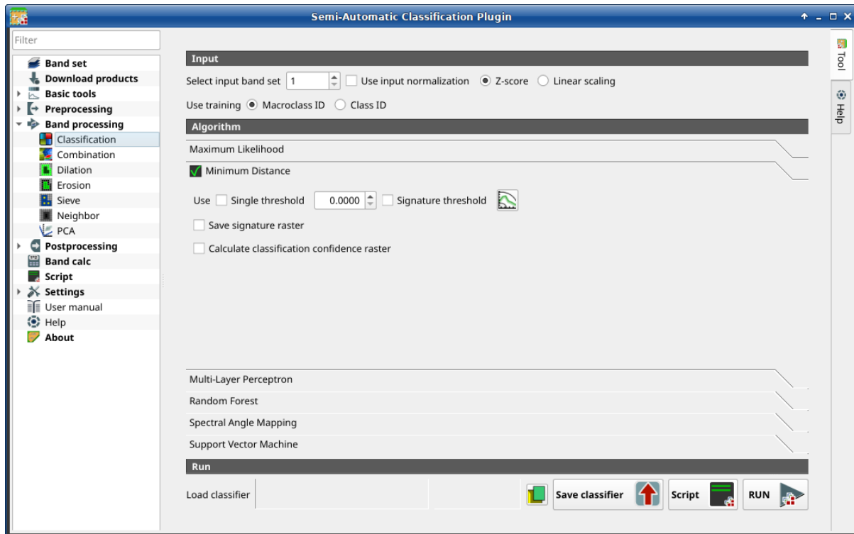
Gambar. 29: Minimum Distance
