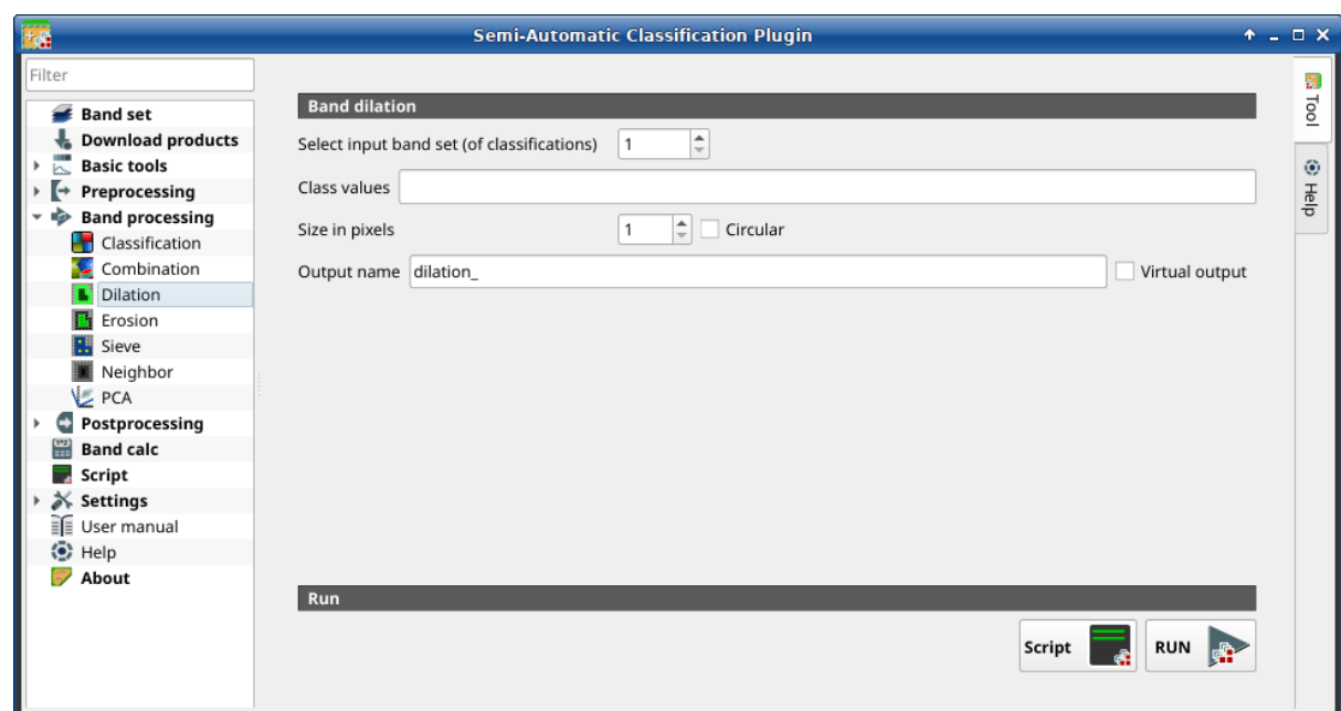
Gambar. 35: Dilation
