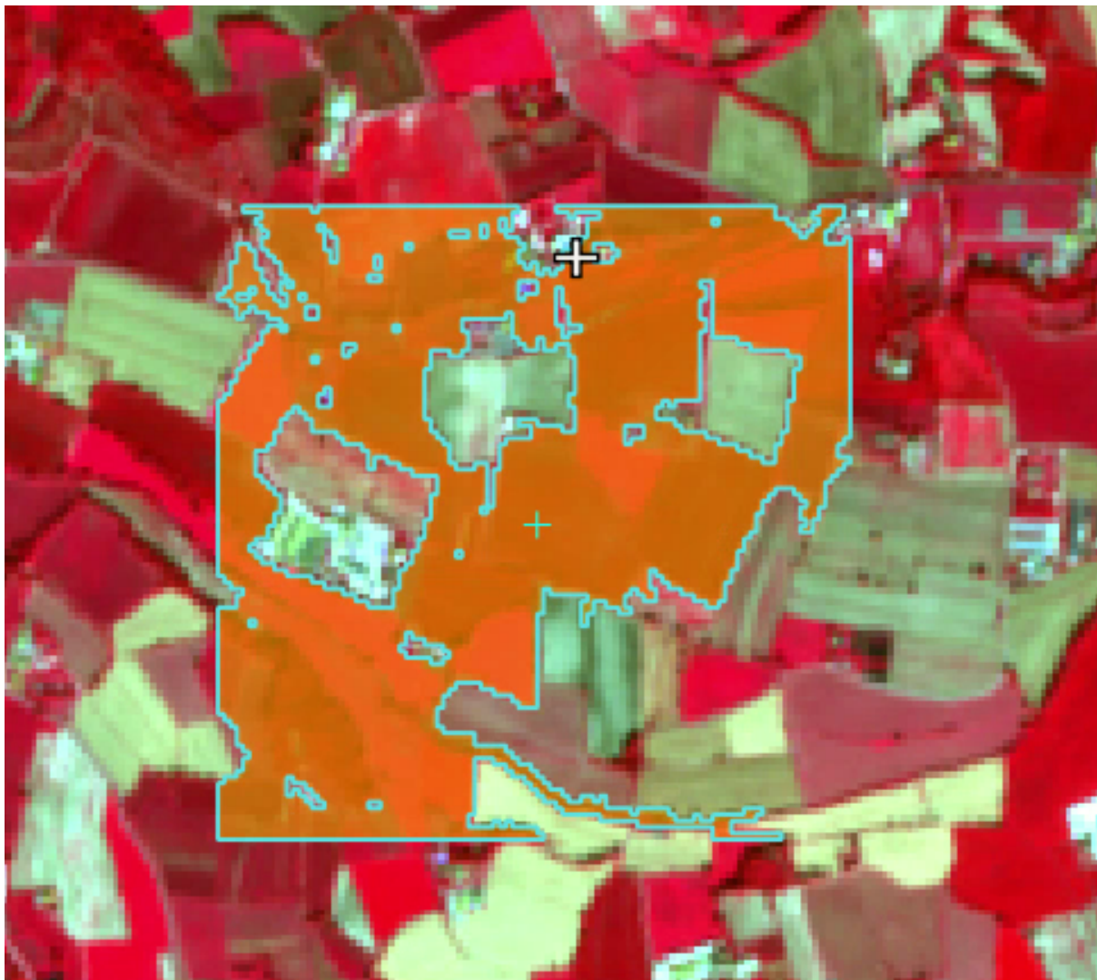
Gambar. 8: Vegetation. Color composite RGB = 7-3-2
