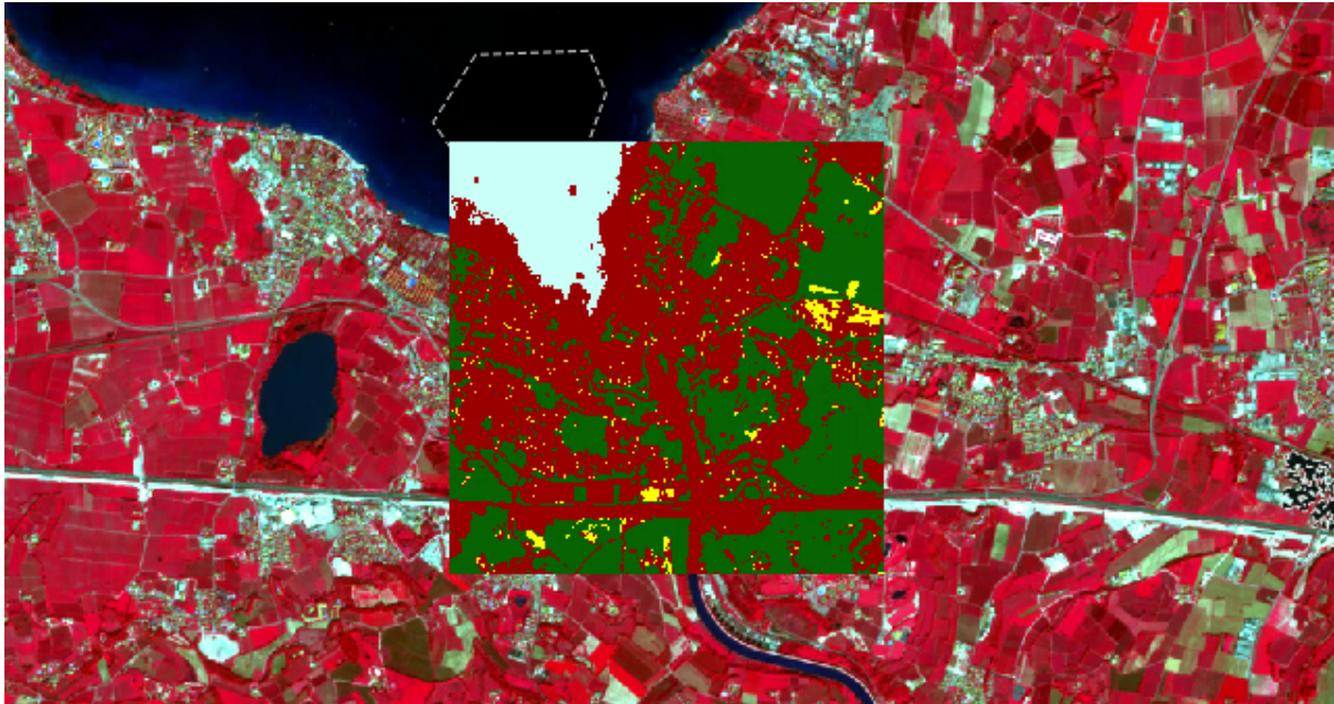
Gambar. 13: Classification preview displayed over the image using MC ID
