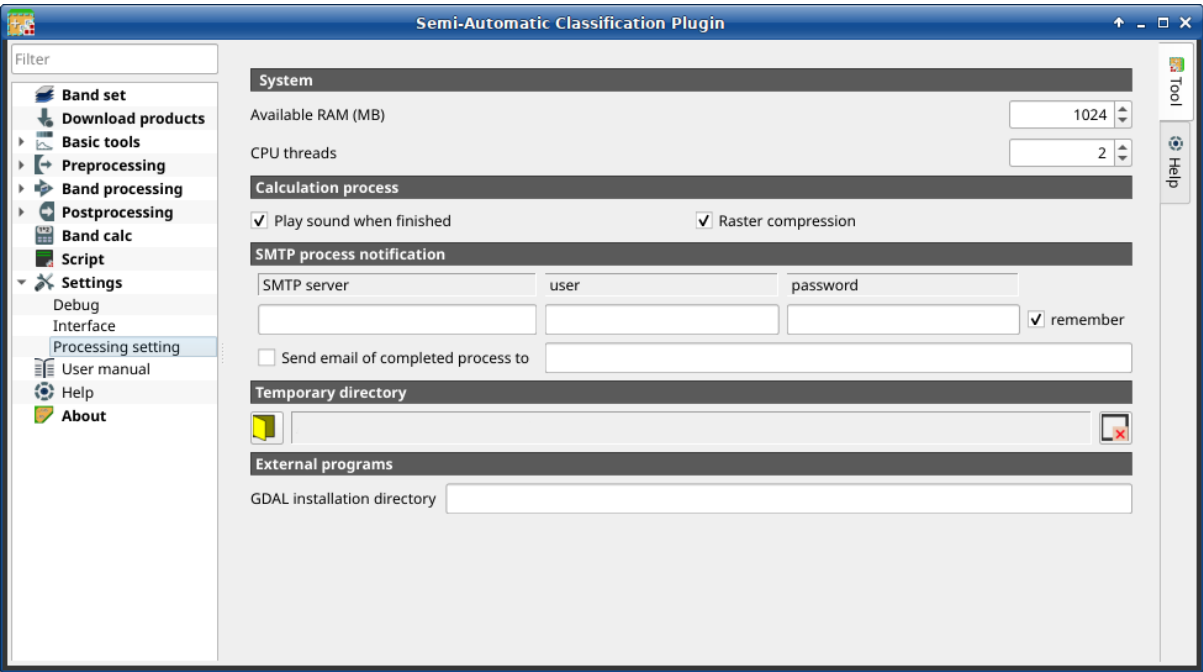
Gambar. 49: Processing
