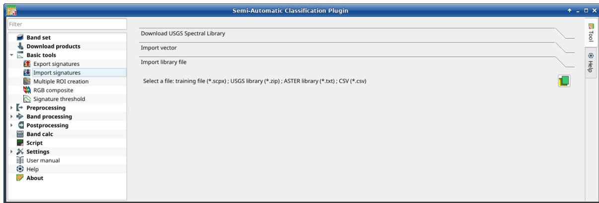
Gambar. 13: Import library file
