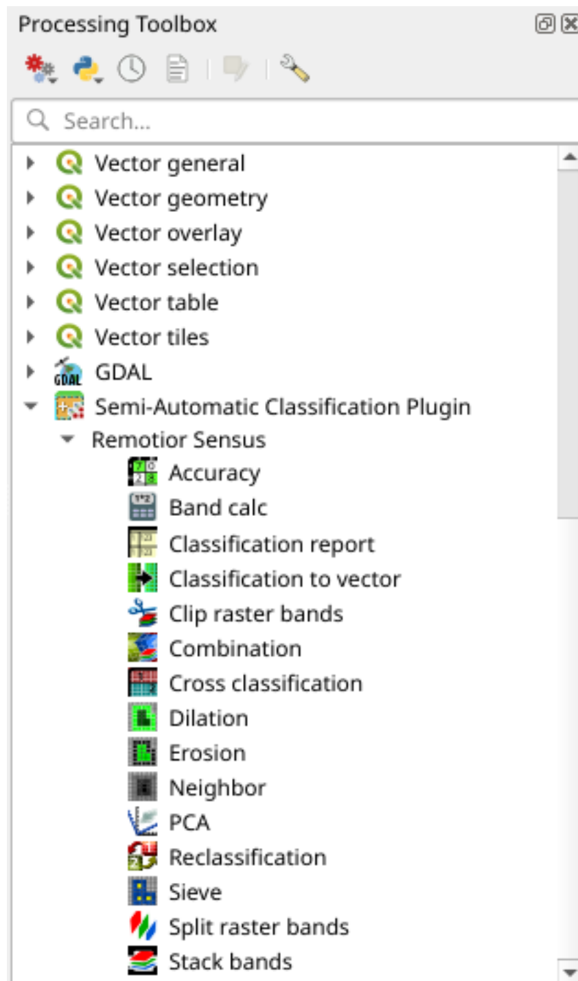
Gambar. 56: Integration in QGIS Processing Toolbox
