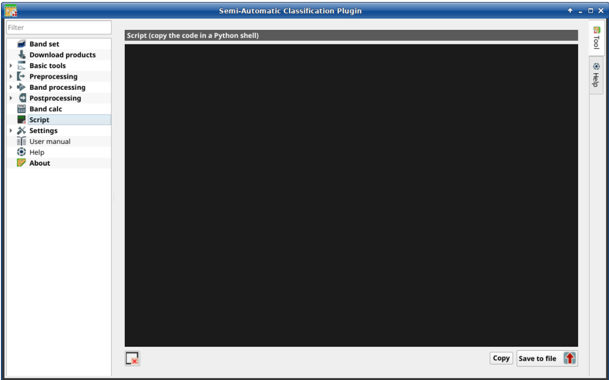
Gambar. 46: Script
