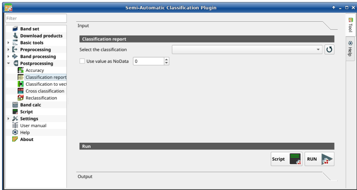
Gambar. 41: Classification report
